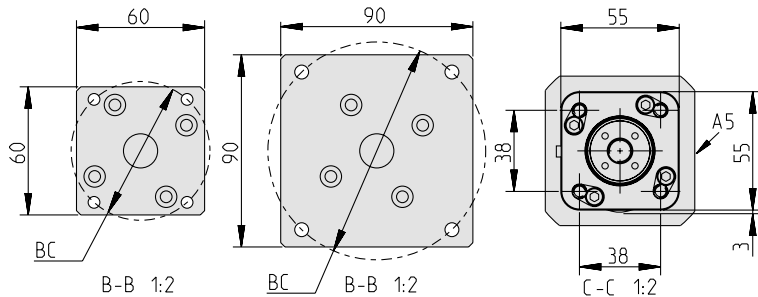
Bride A
