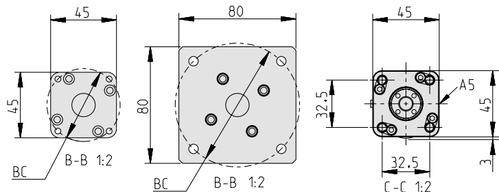
Bride A
